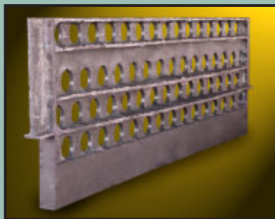
Tube Sheet (ASTM A-560 50Cr-50Ni Nb)
